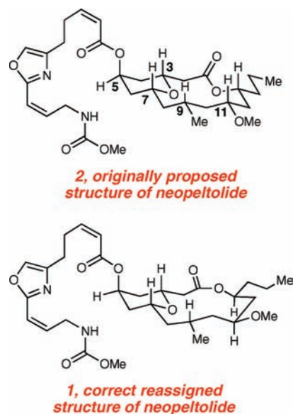
Figure 1. Neopeltolide structures.
